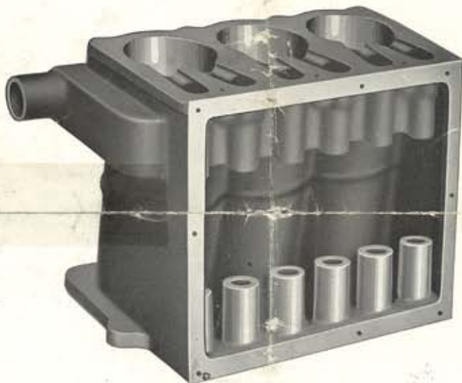
Cylinder Block
