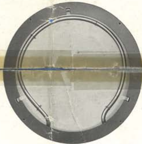
Refractory Lined Pan With Superheater Coil.
