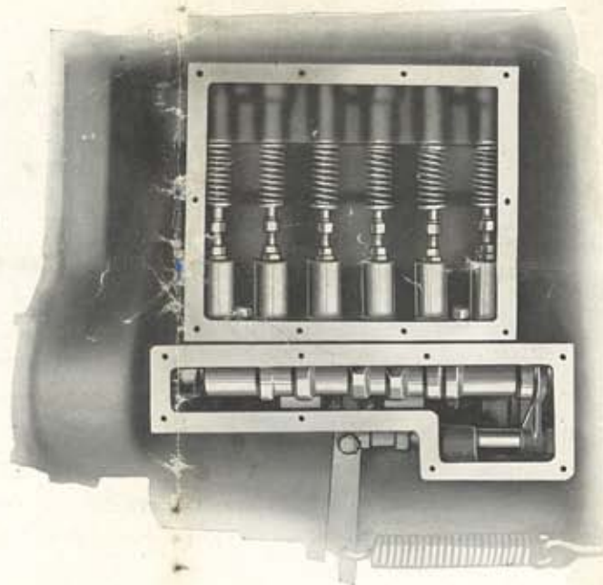
Engine Assembly, showing valves, cam action and accessibility
