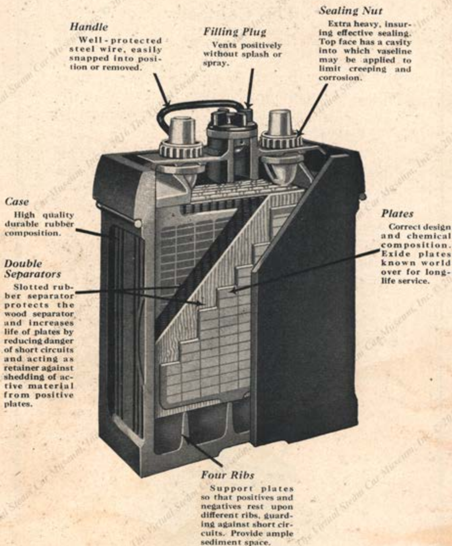
Sectional View of a Typical Exide Automobile Battery Showing Construction Details
